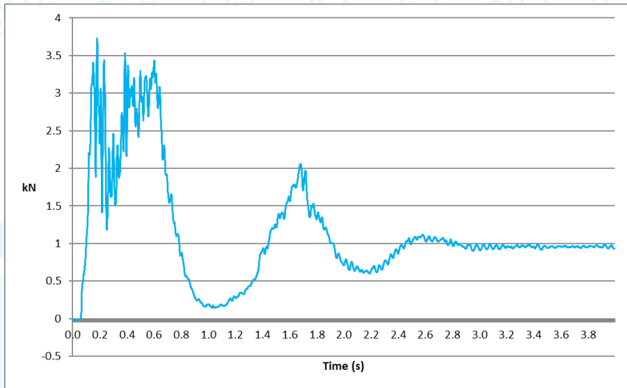
Figure 2 – Dynamic performance: Graph of arrest force vs. time
